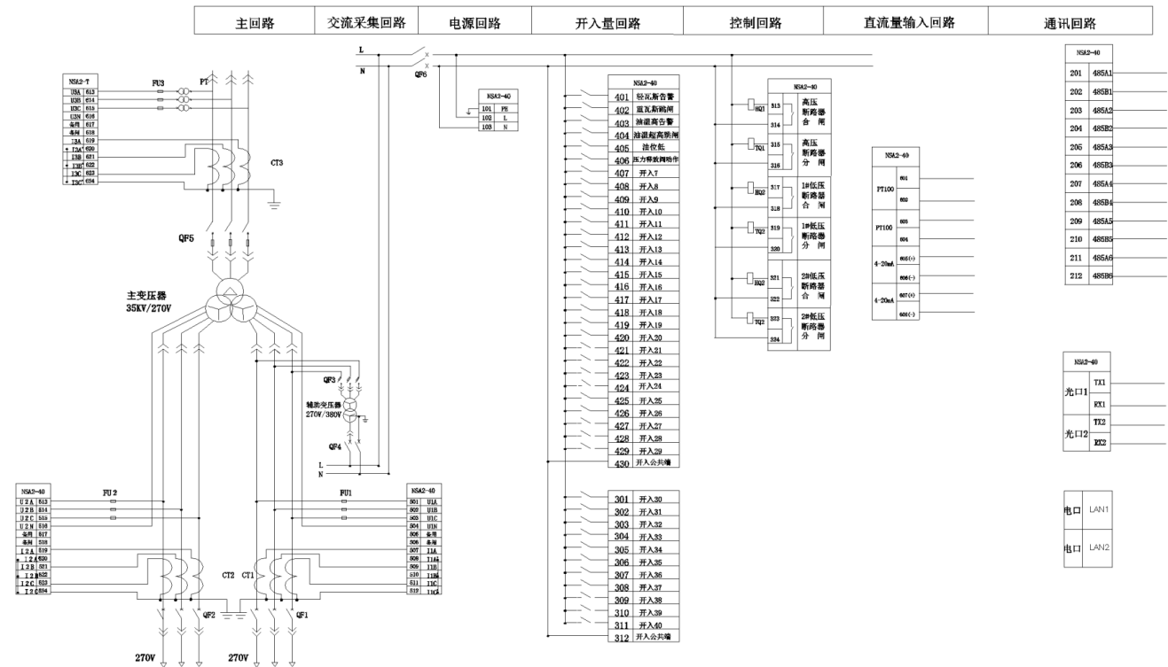
Typical secondary wiring diagram (example, labels in Chinese)
