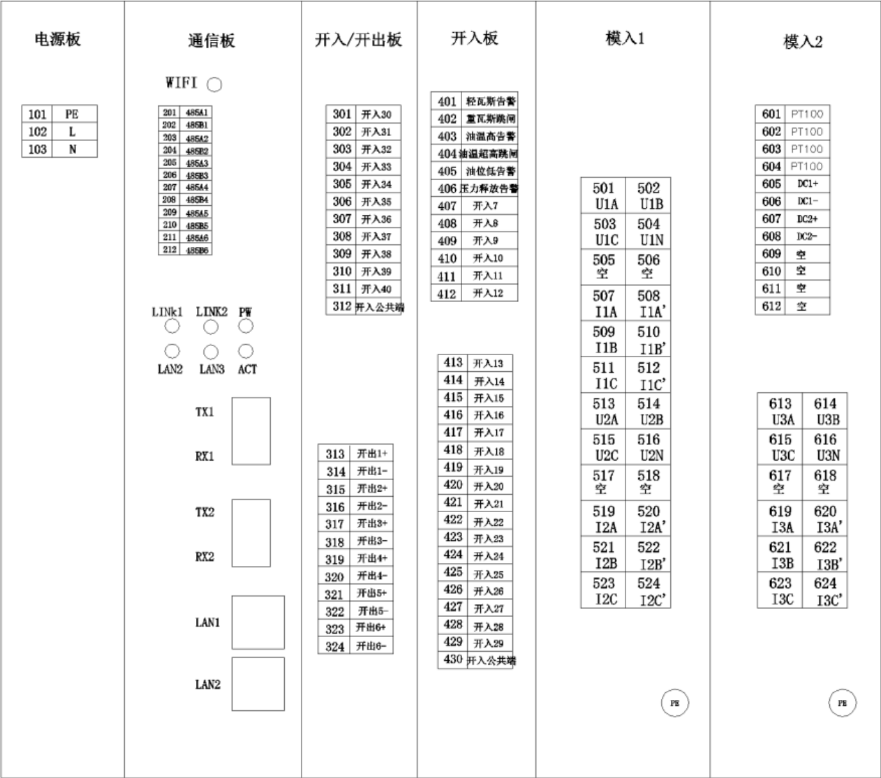
Typical rear terminal diagram (example, labels in Chinese)
